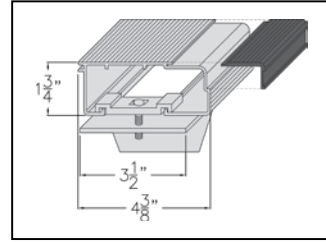
2" x 5" w/nosing
