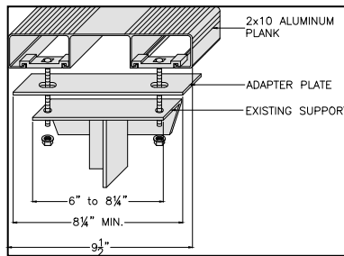
Seat Adapter Plate
